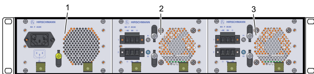
Figure 9: M4-POWER power unit chassis, front side of the device (mounting with up to 3 power units) 1 - Power unit 1 2 - Power unit 2 3 - Power unit 3
