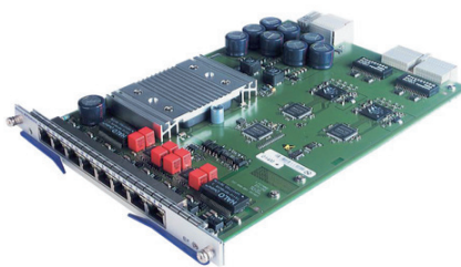
M4-FAST 8TP-RJ45-PoE
